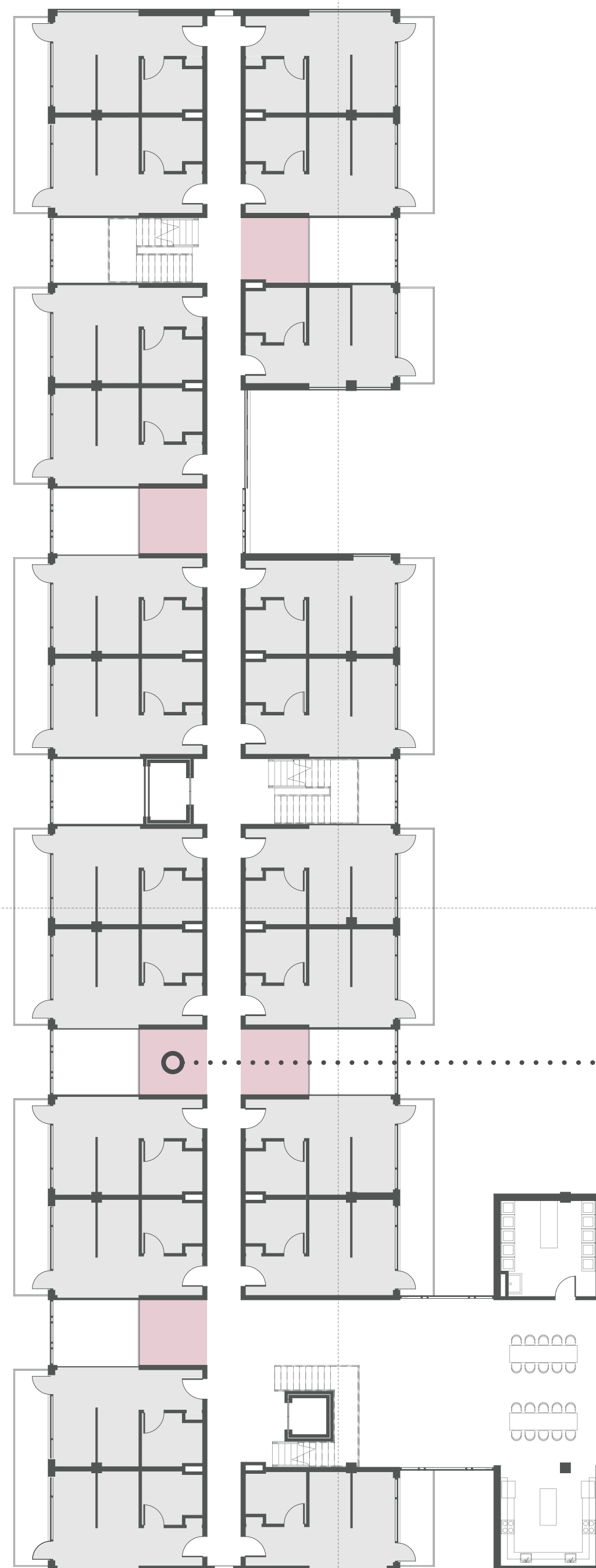
THIRD FLOOR PLAN 1/32"
