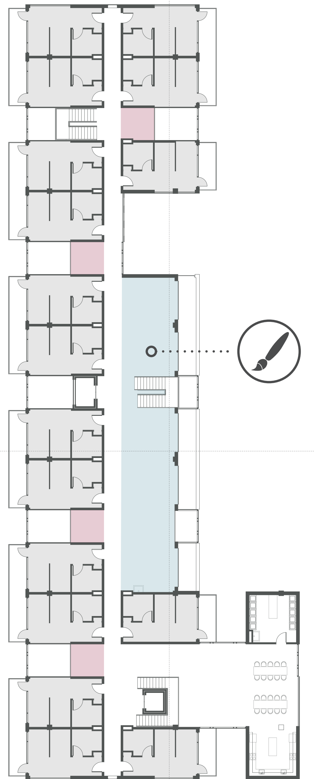
FOURTH FLOOR PLAN 1/32"
